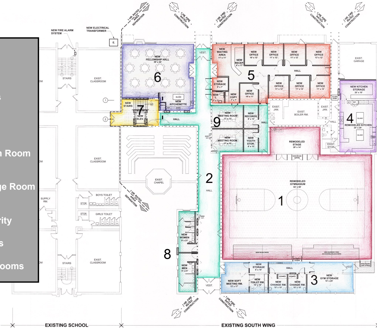
CONCEPTUAL FIRST FLOOR PLAN SCALE = 3/32" = 1'-0"
